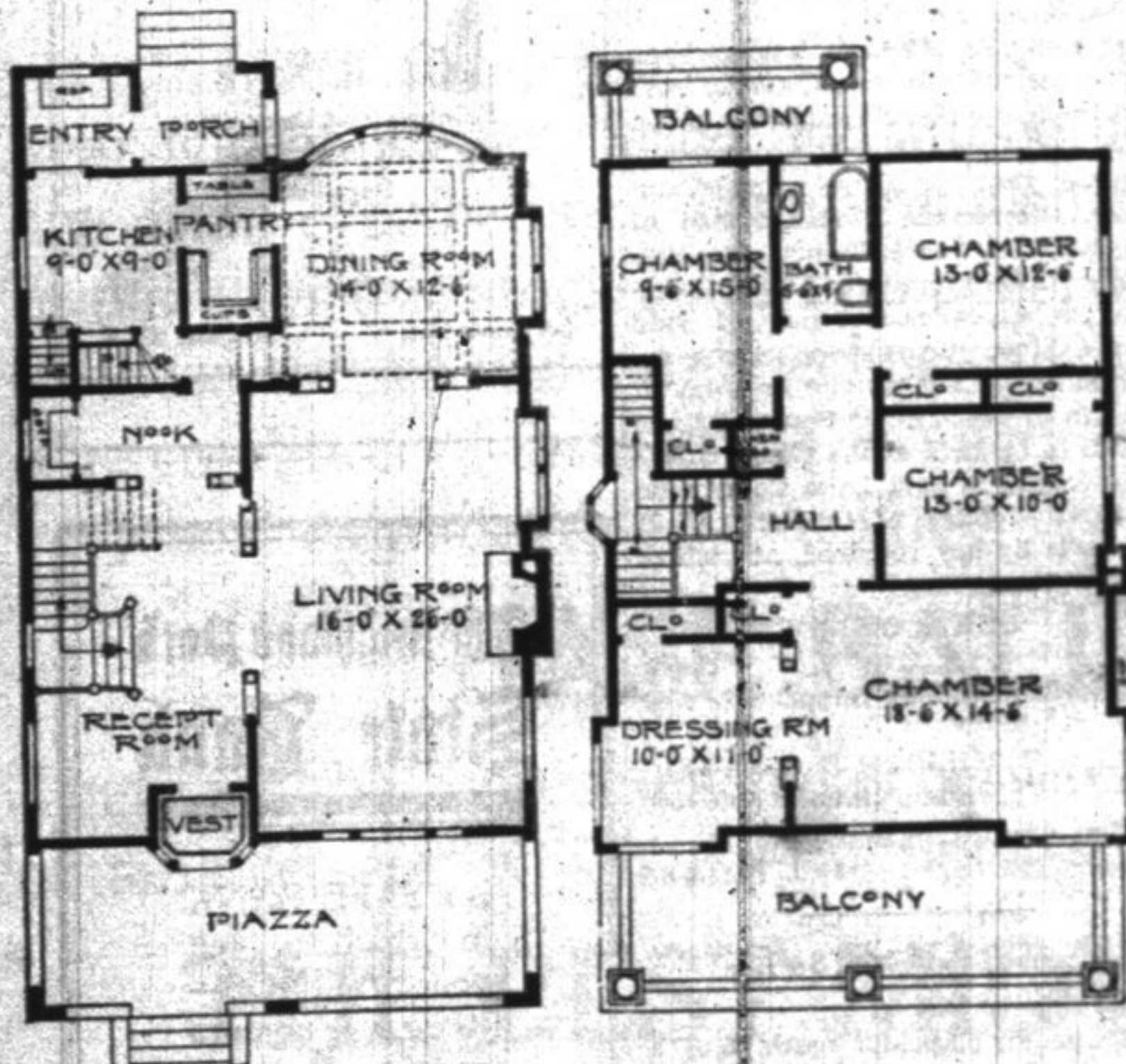
FIRST FLOOR PLAN. SECOND FLOOR PLAN.
