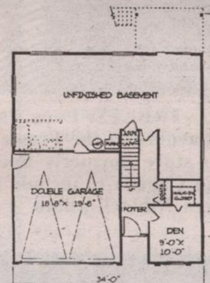
BASMENT FLOOR PLAN 886 SQ. FT.
