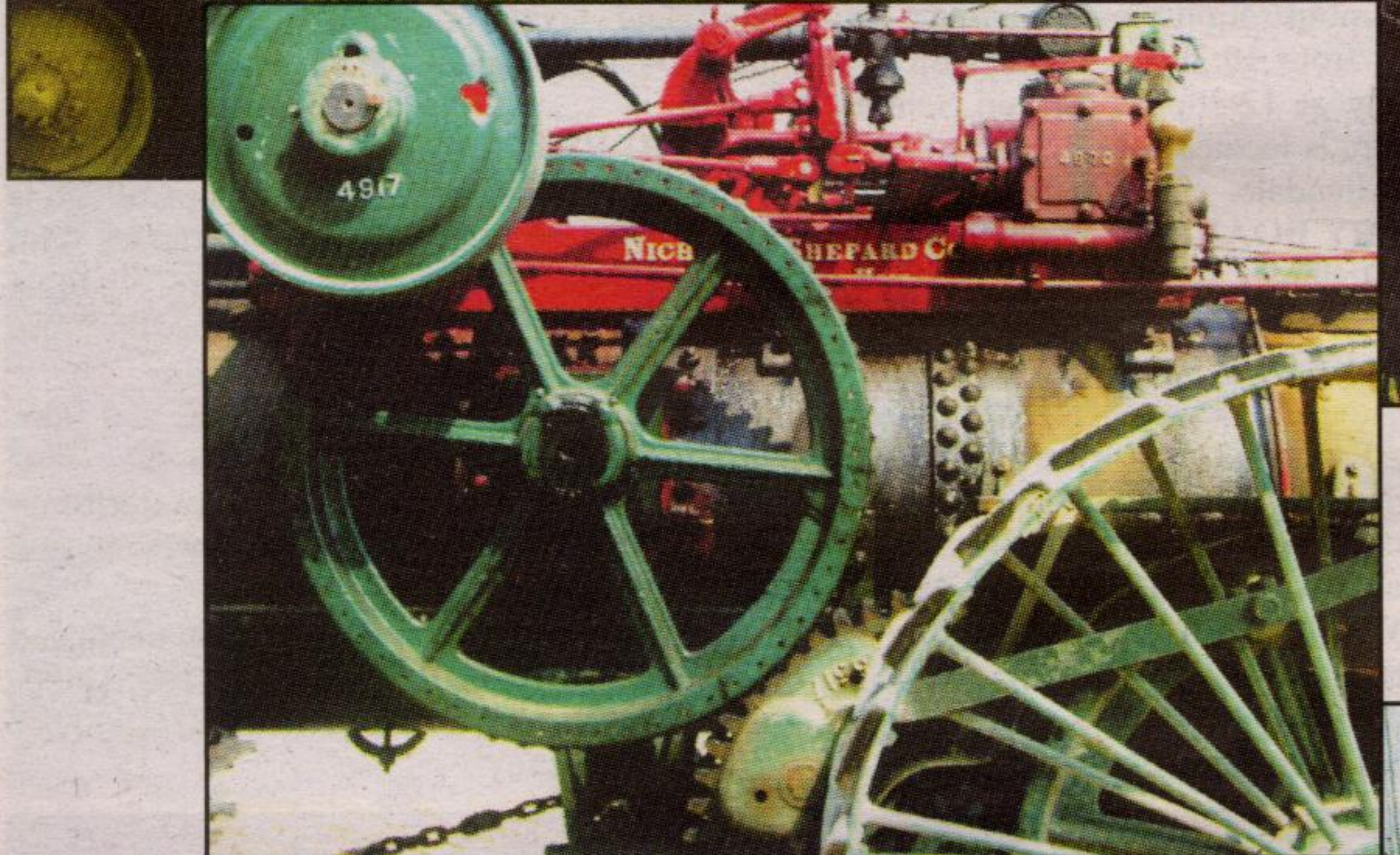
Steel Pulleys and gears from a 40,000 lb steam Tractors – some of the largest and heaviest ever made.
