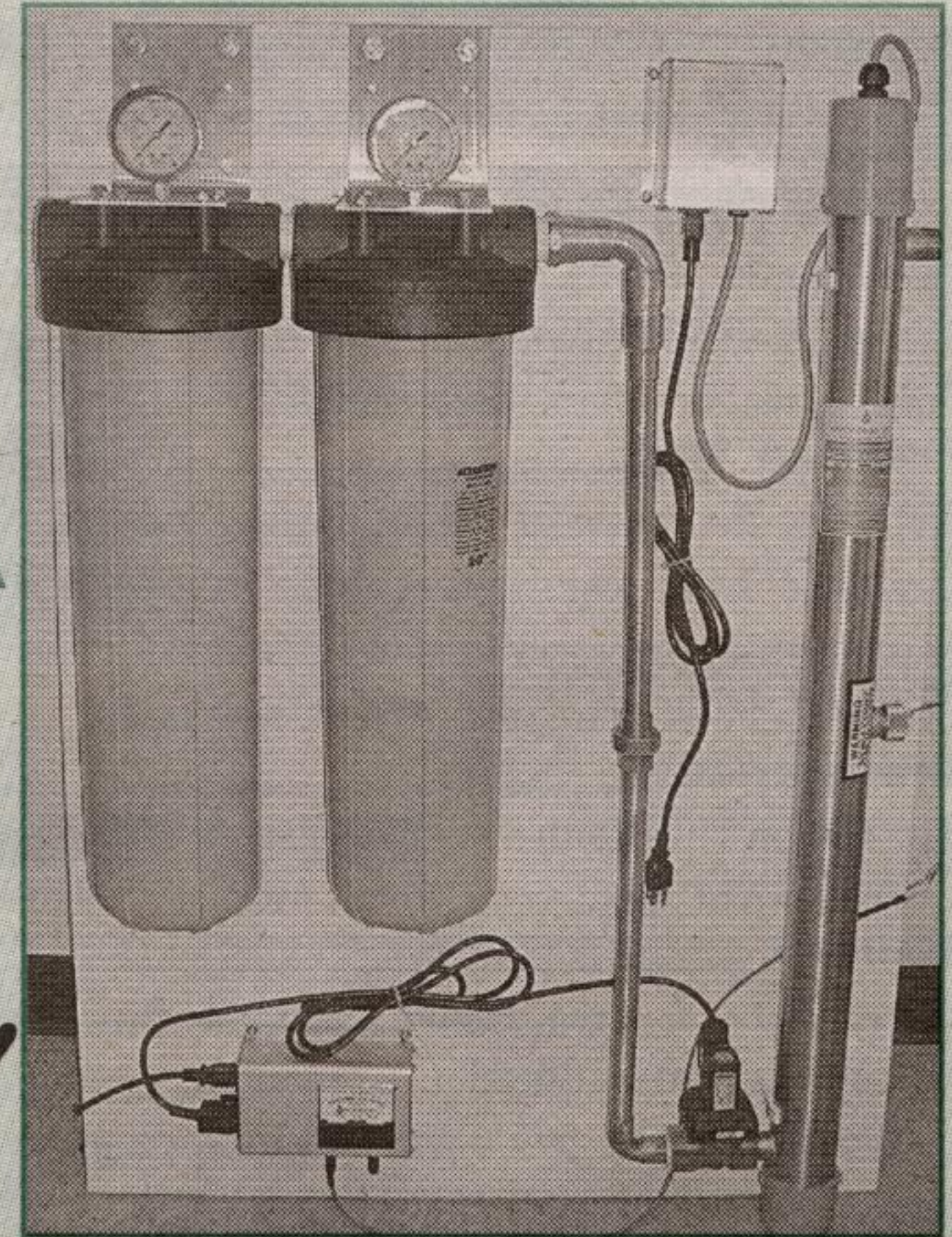
Filtration System
