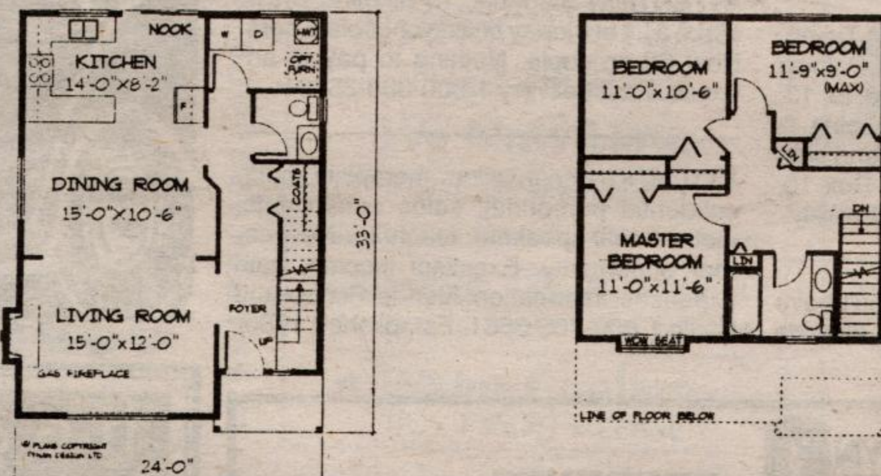
MAIN FLOOR PLAN 740 SQ. FT. UPPER FLOOR PLAN 592 SQ. FT. TOTAL FLOOR PLAN 1332 SQ. FT.
