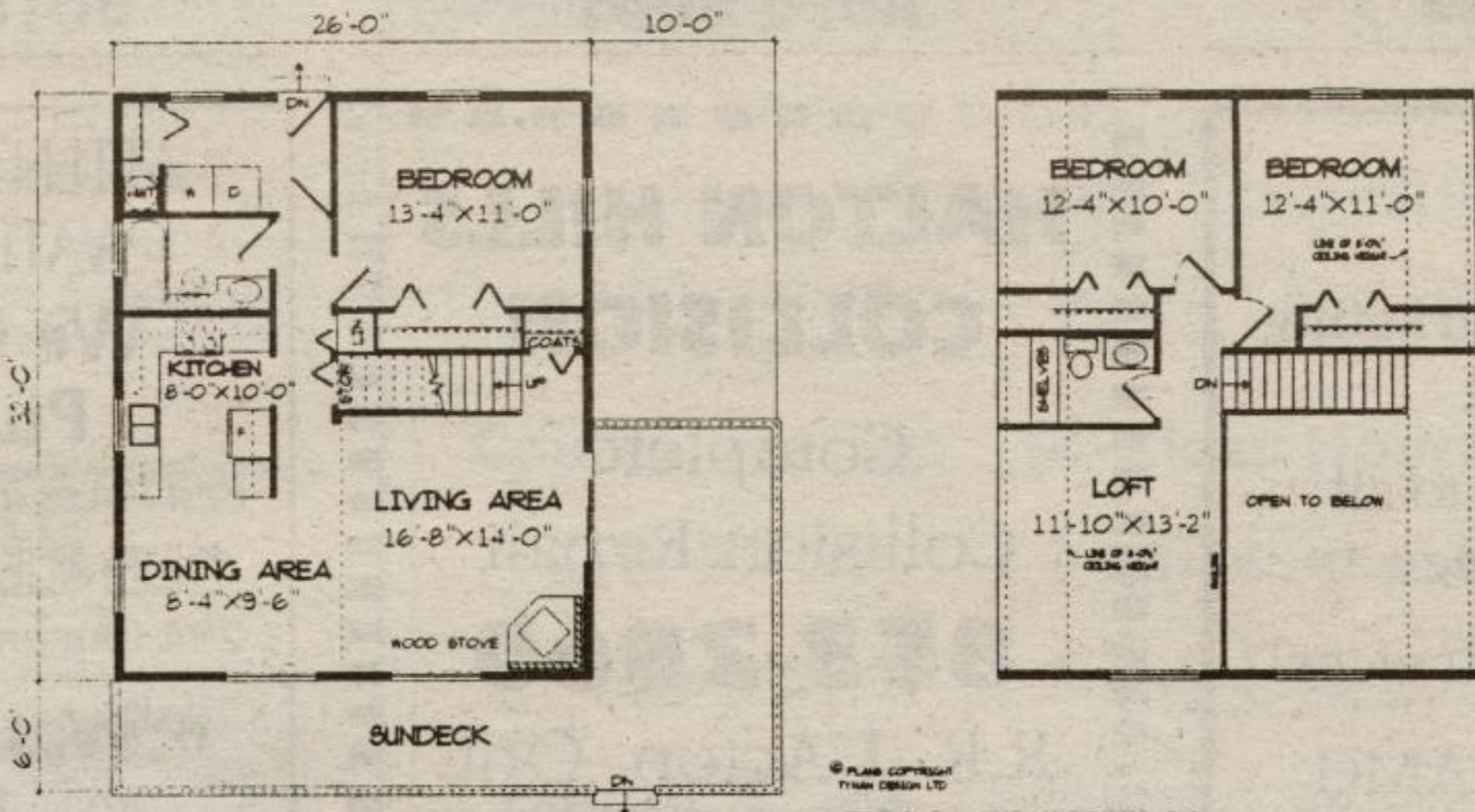
MAIN FLOOR PLAN 832 SQ. FT. UPPER FLOOR PLAN 589 SQ. FT. TOTAL FLOOR AREA 1421 SQ. FT.
