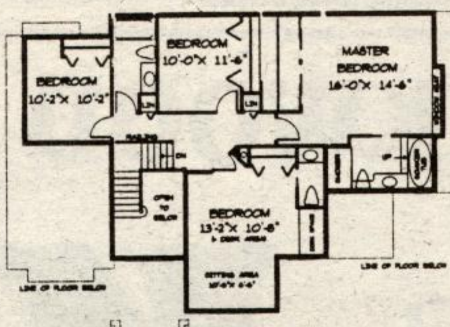
UPPER FLOOR PLAN 1185 SQ. FT.
