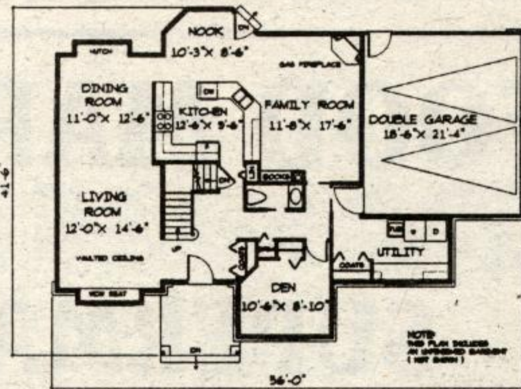
MAIN FLOOR PLAN 1285 SQ. FT.
