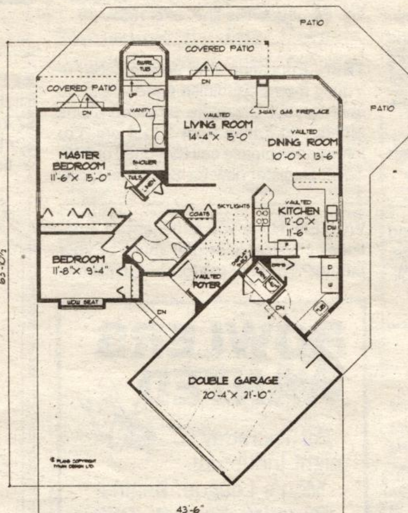
MAIN FLOOR PLAN 1377 SQ. FT.
