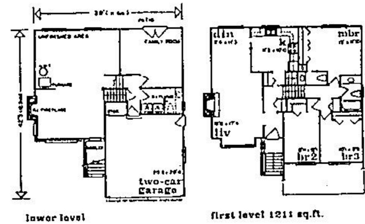
PLAN NO. 81-1211 © Copyright 1981, Small Home Design, All rights reserved.
