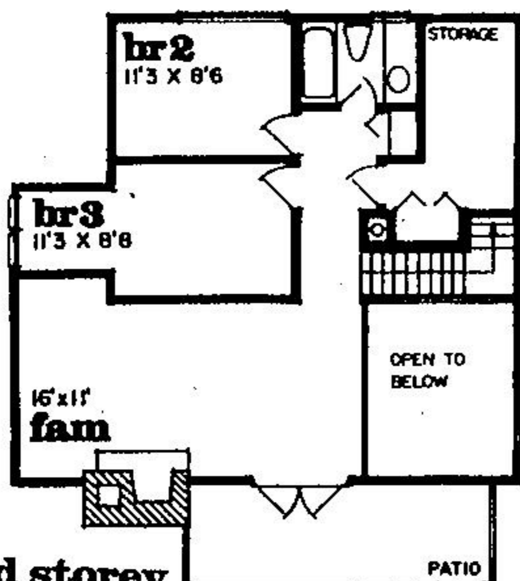
first storey 1110 sq. ft.
