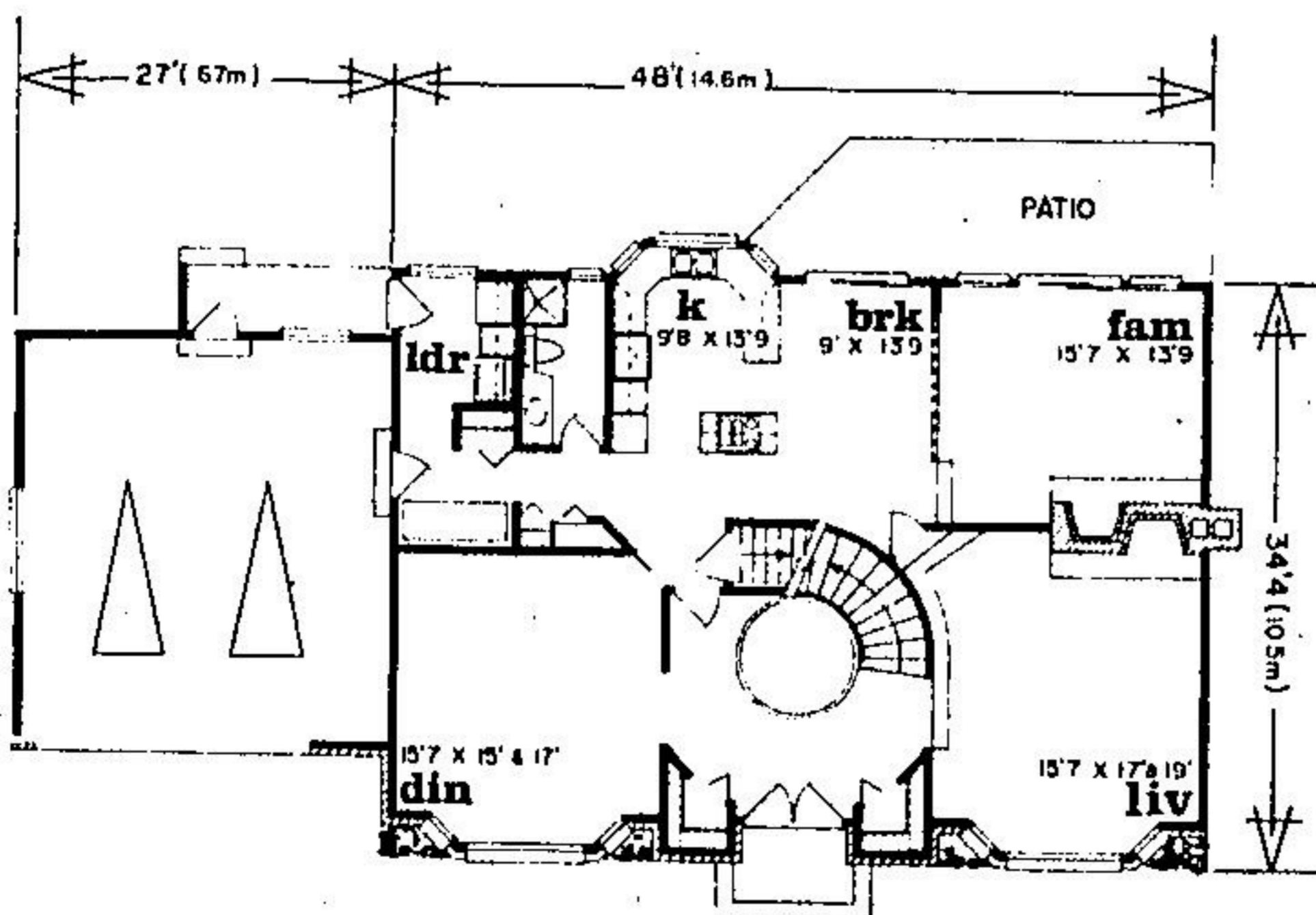
first storey 1608 sq. ft.
