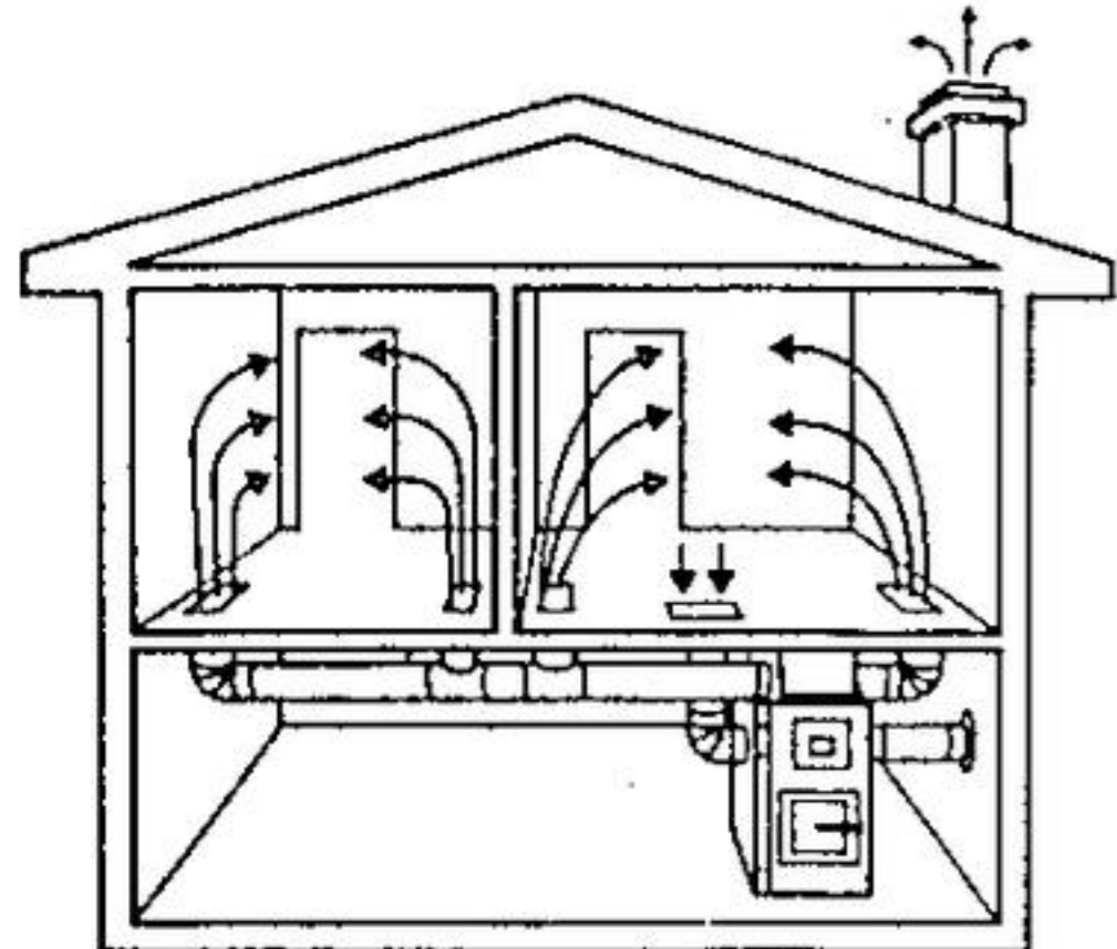
Heating the entire house is possible with a furnace and suitably arranged ducts.
