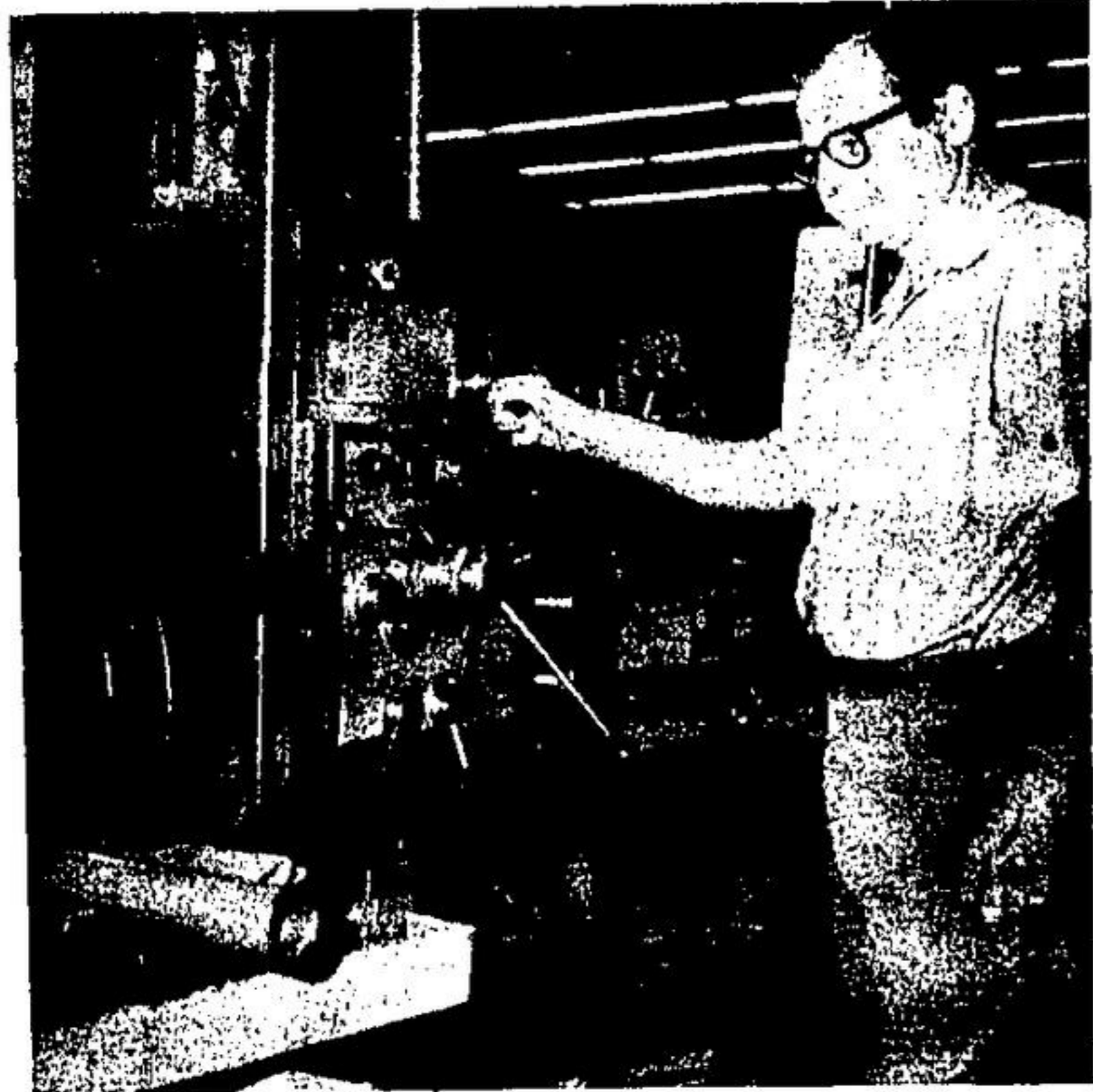
Machinist, Peter Pelkman of Brampton, operates a horizontal boring mill at Yoder Equipment of Canada on Todd Rd. A very versatile machine the boring mill performs castings and welding operations on segments.
