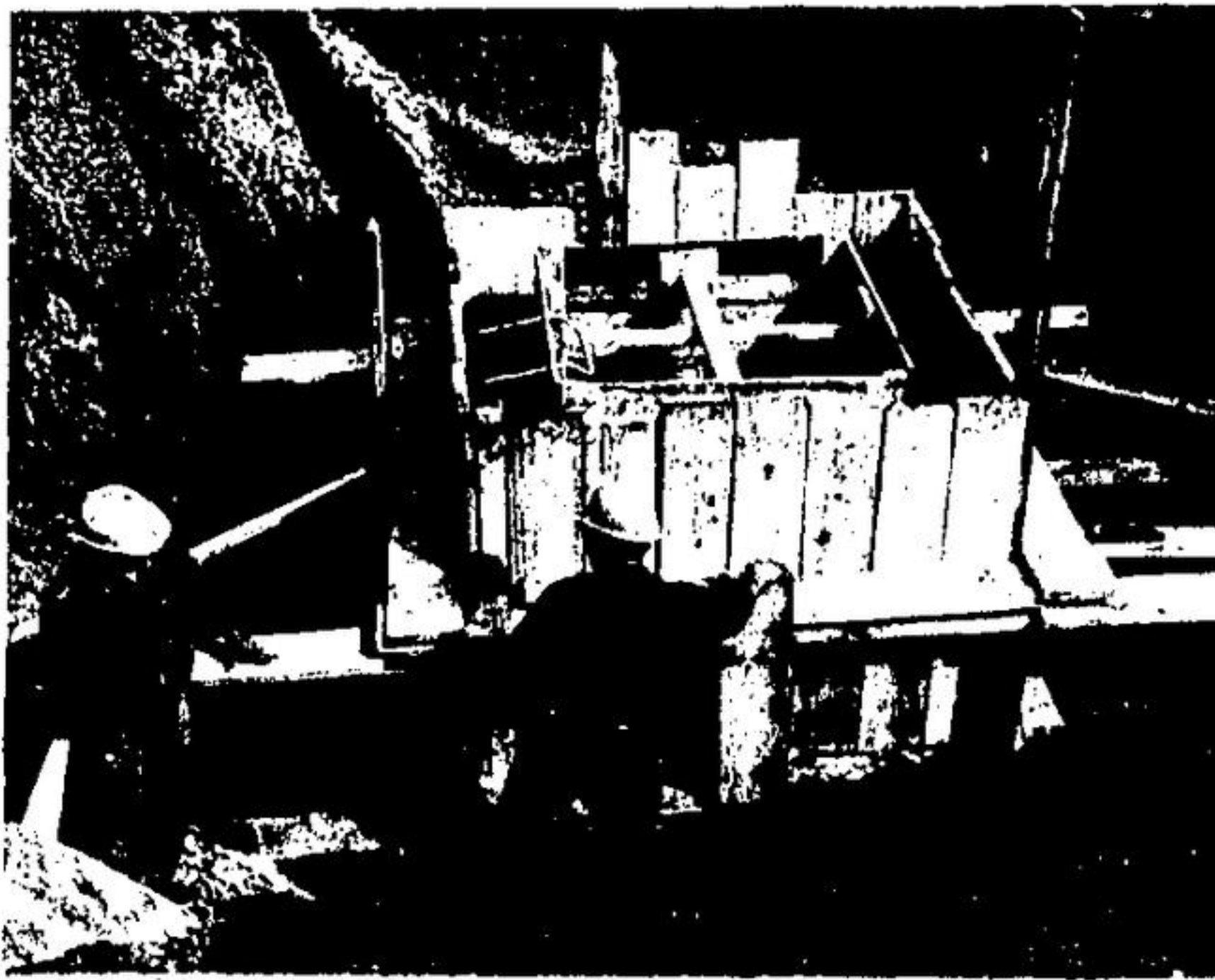
EMPLOYEES OF En-San of Toronto build forms for concrete manholes, part of the storm sewer system now being constructed at the CN Georgetown station grounds. The storm sewer is buried deep in the sandy soil of the station property. GO Train preparations are responsible for the flurry of activity now abuilding at the station.
