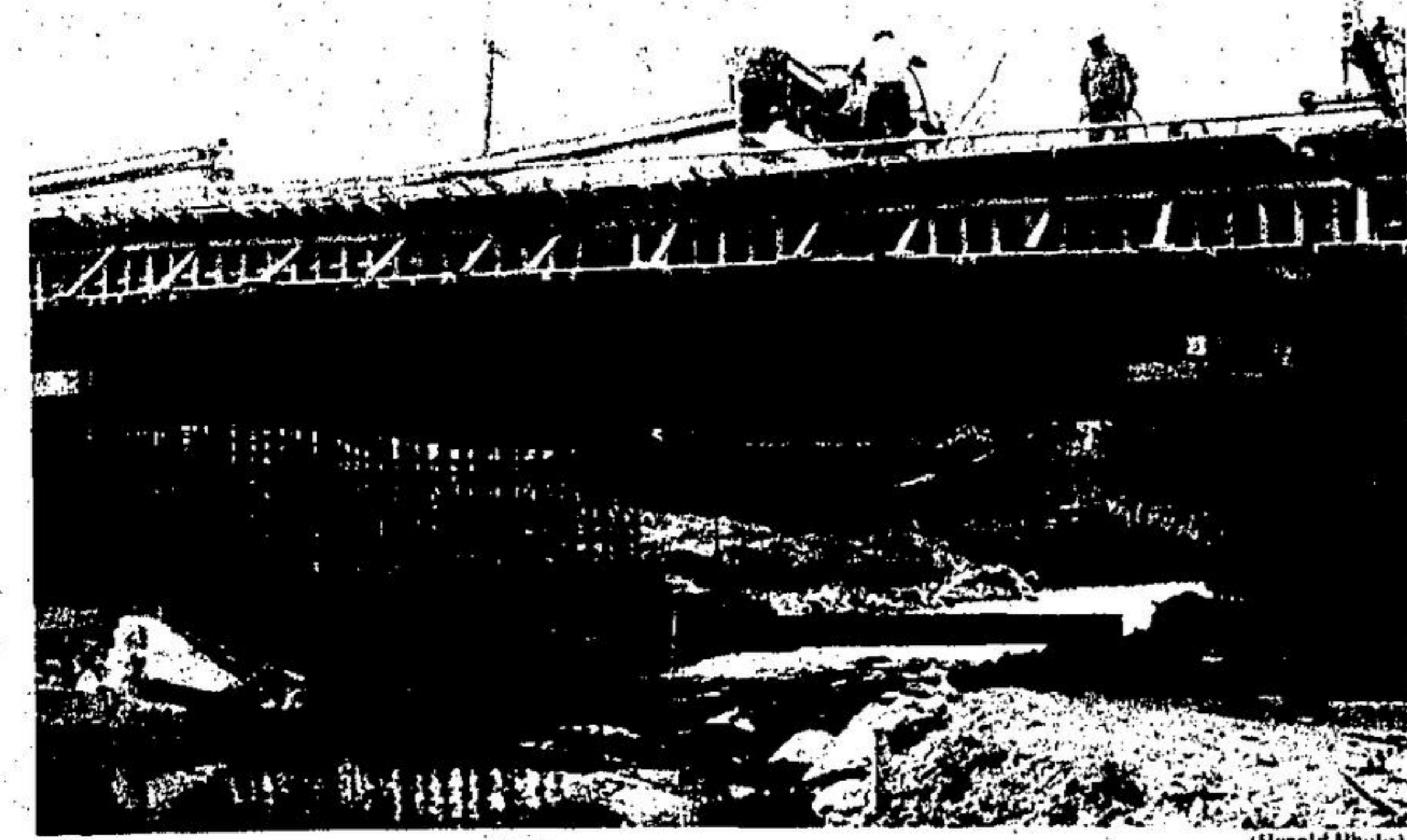
As the summer progresses, a new bridge across the west branch of the Credit River at Norval. Concrete for the main bridge structure has been poured. The bridge will straighten the approach of Highway 7 into Norval from the east. The river flows through a narrowed channel beneath the new structure.
