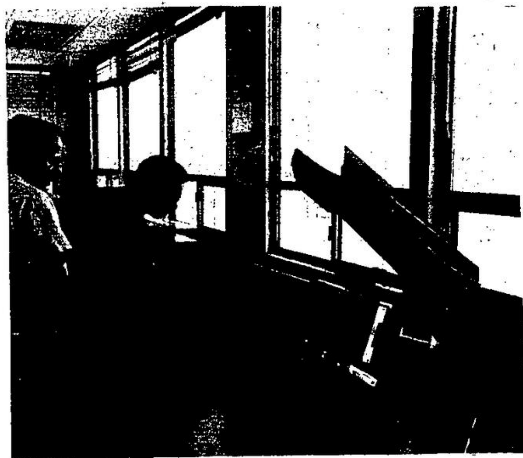
Engineering Technologist Rod Keizer (foreground) and Electrical Engineer Al J. Reed, are setting up a test on the console in the field experimental lab using the big surge generator in the grounds outside. Mr. Reed is
