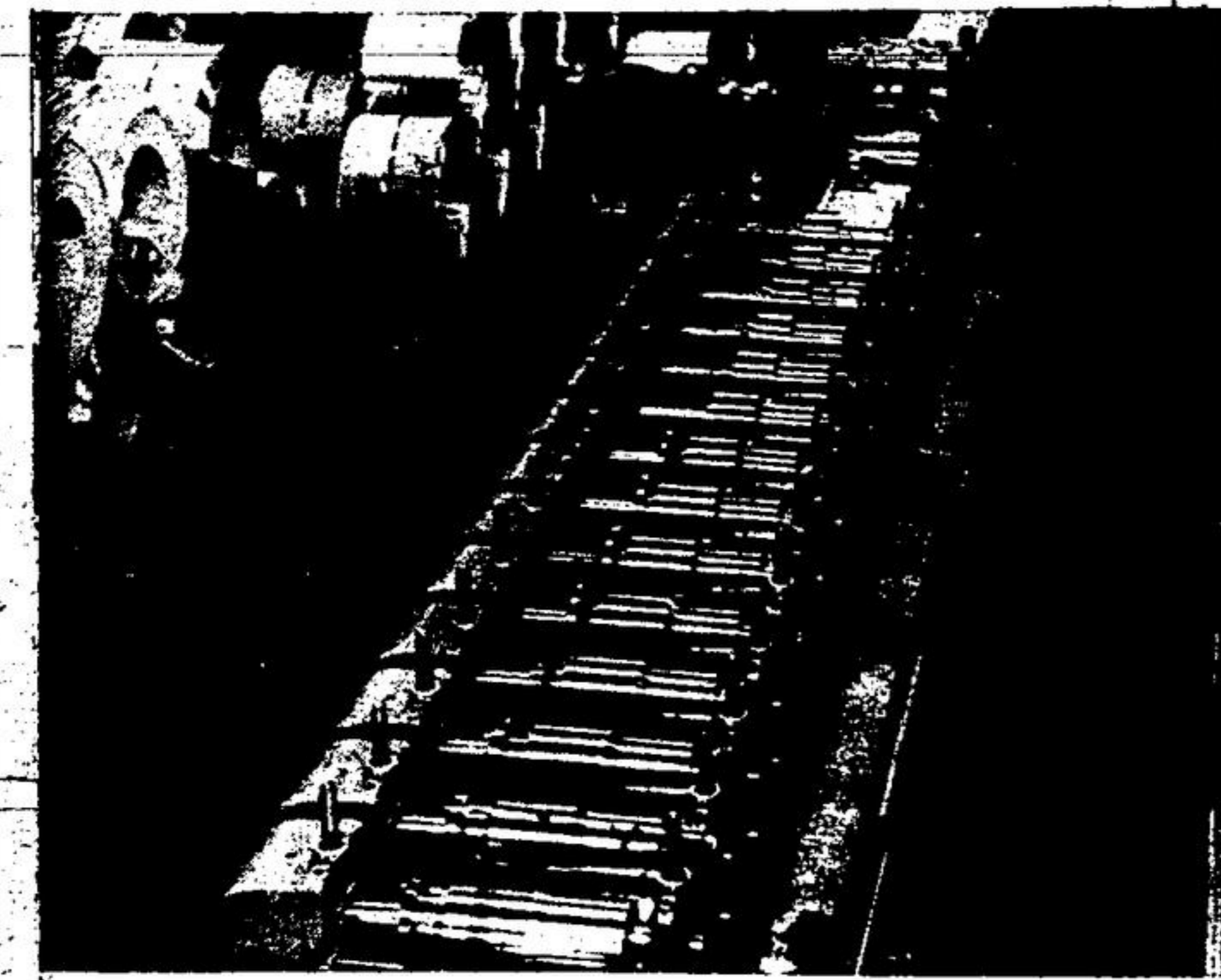
Yoder M-2 roll forming machine with flying cutoff, used in the manufacture of building siding. This unit is capable of making siding of pre-painted aluminum or stainless steel.
