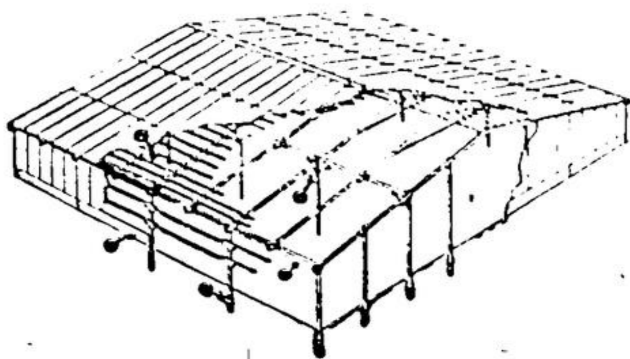
Pictured above is a Beaver Pole-Type Lounging Barn showing details of the Beaver engineered method of construction.
