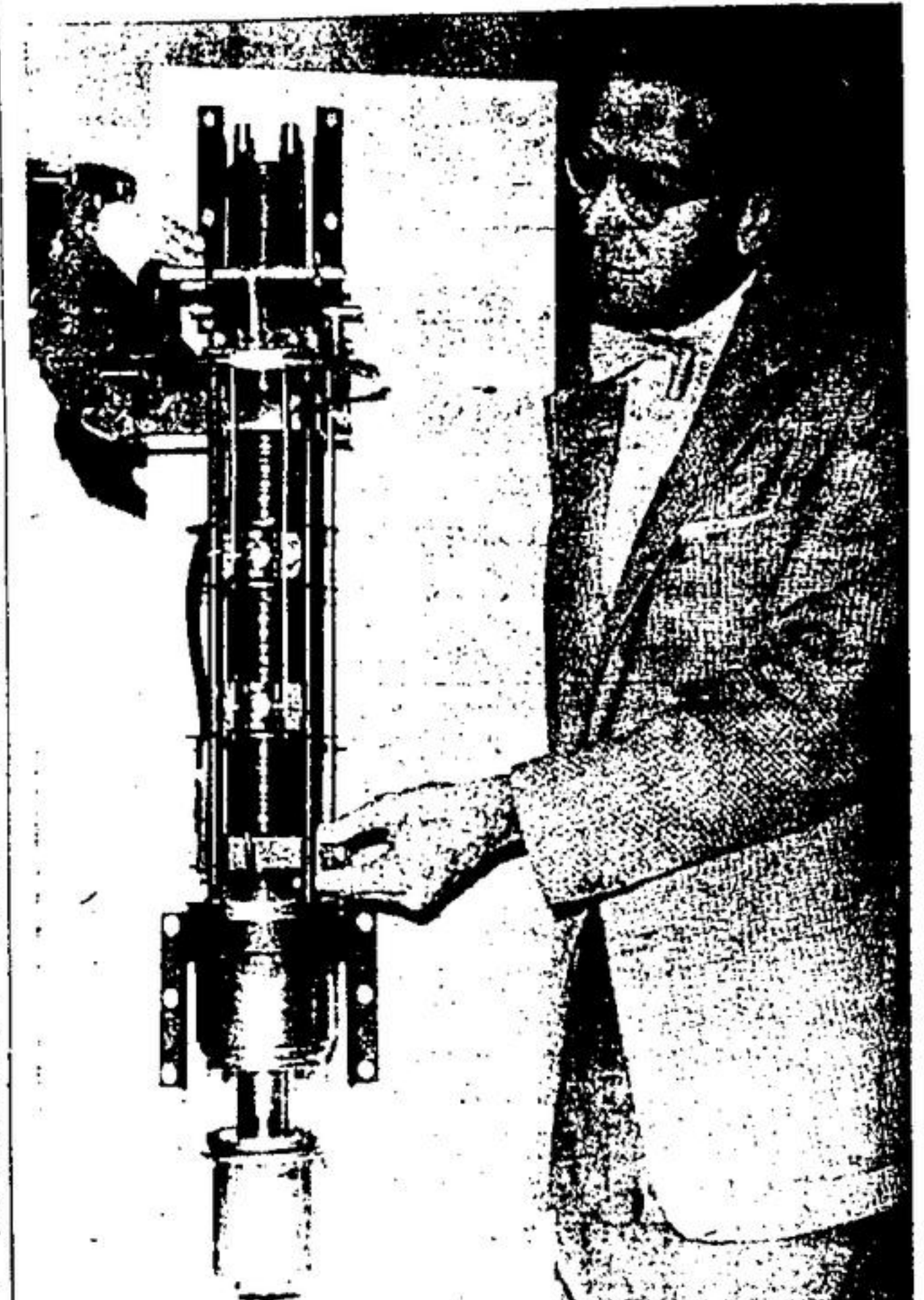
This klystron generates over one million watts of radio-frequency power in very short bursts of energy for radar applications. Paul Corbell, engineering and sales manager of Varian Associates plans to have this pulse klystron in small quantity production here next year.
