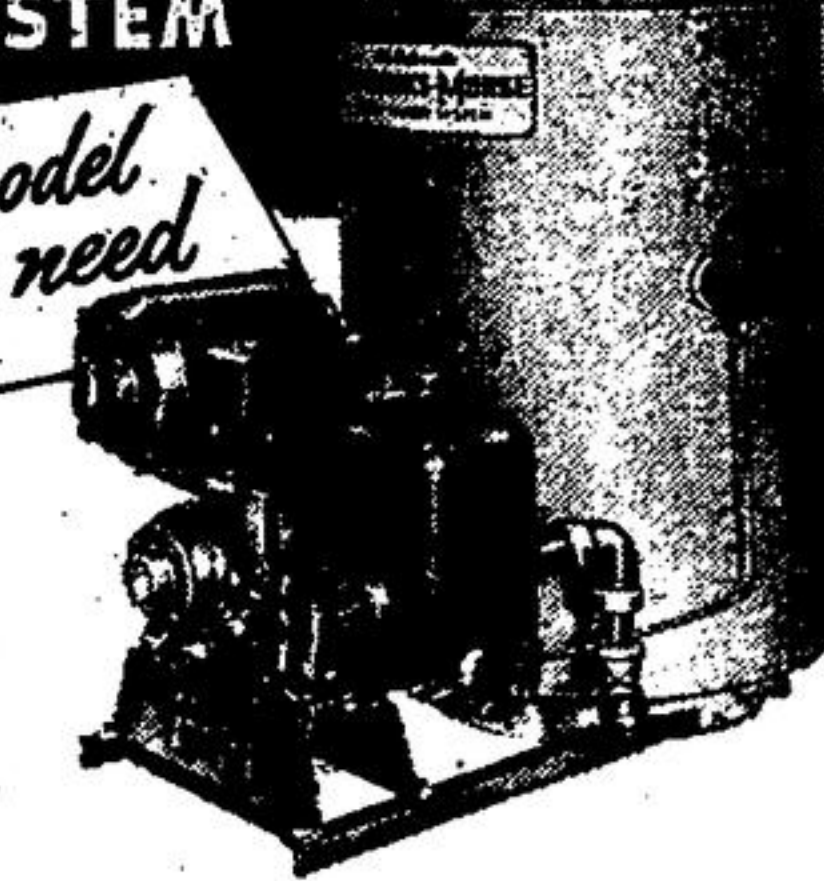
Model 425M-30 Fairbanks-Morse Shallow Well Water System, Capacity 400 gallons per hour. Self-oiling, Double-acting, Self-priming.
