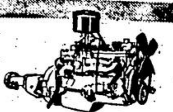
Plymouth's 97-h.p. engine has plenty of zip. Its 4-way carburetion and high (6.7 to 1) compression ratio give you peak performance at all speeds.
