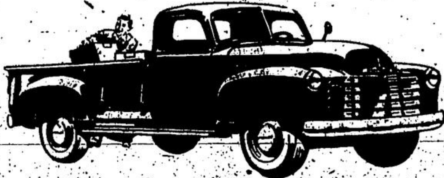
PICKUP MODELS Model 1424-125 1/2-inch wheelbase, Maximum G.V.W. 6000 lbs. Other models available: 1424 — 137-inch wheelbase, Maximum G.V.W. 6700 lbs.; 1314 — 116-inch wheelbase, Maximum G.V.W. 4600 lbs.
