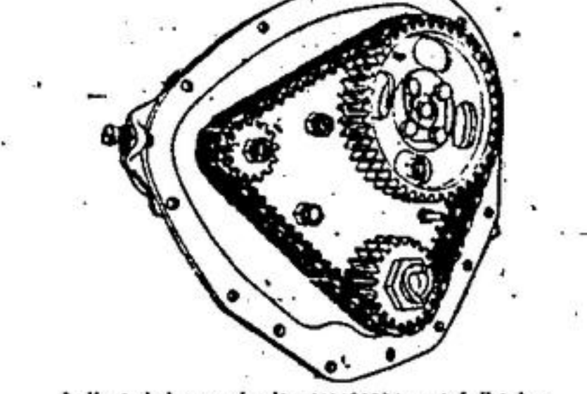
A silent chain, running in a constant spray of oil, takes the place of the usual timing gears, and thereby contributes to the quietness of the Light-Six motor.
