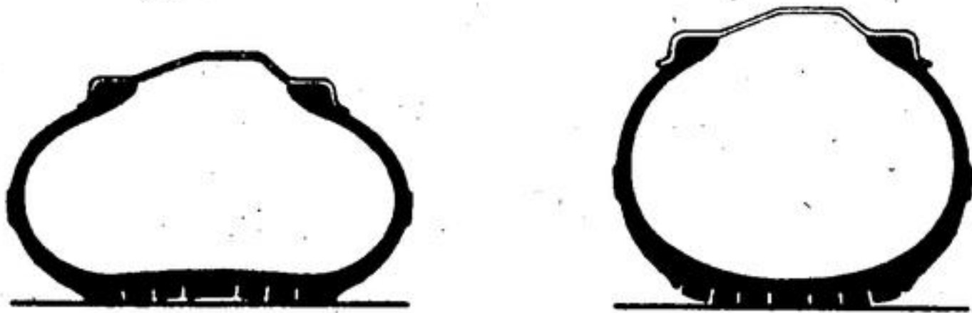
Proper inflation is vital to tire safety. An underinflated tire (left) causes extreme flexing and builds up excessive heat, running the risk of failure. It also causes rapid wear on the outer edges. Overinflation (right) makes tires run hard and may cause impact damage, weakening of the carcass and excessive wear in the centre. Either underinflation or overinflation results in improper contact with the road.
