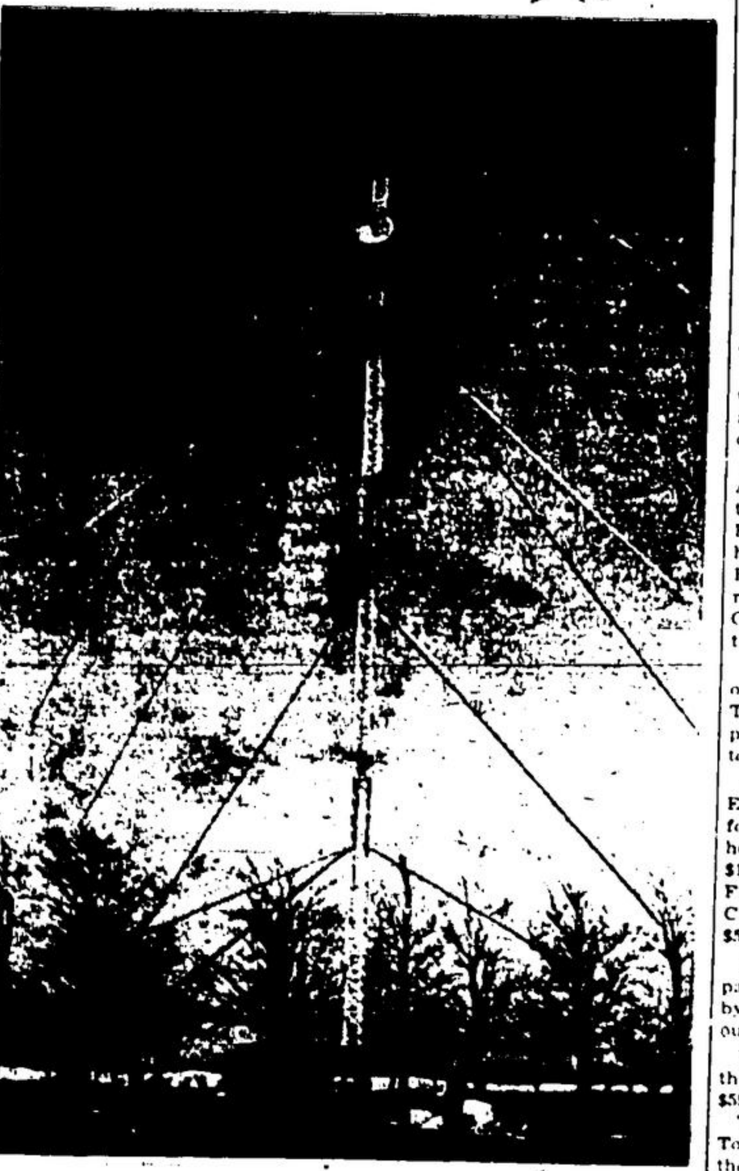
TRANSMITTING MICRO-WAVE SIGNALS is this 140-foot tower at Milton Heights. From Buffalo to Fonthill, to Milton and then to Toronto go these signals which are indicating that television could be successfully transmitted from these towers. The direct route across Lake Ontario is too great for a single radio link. —Photo courtesy Bell Telephone Co.
