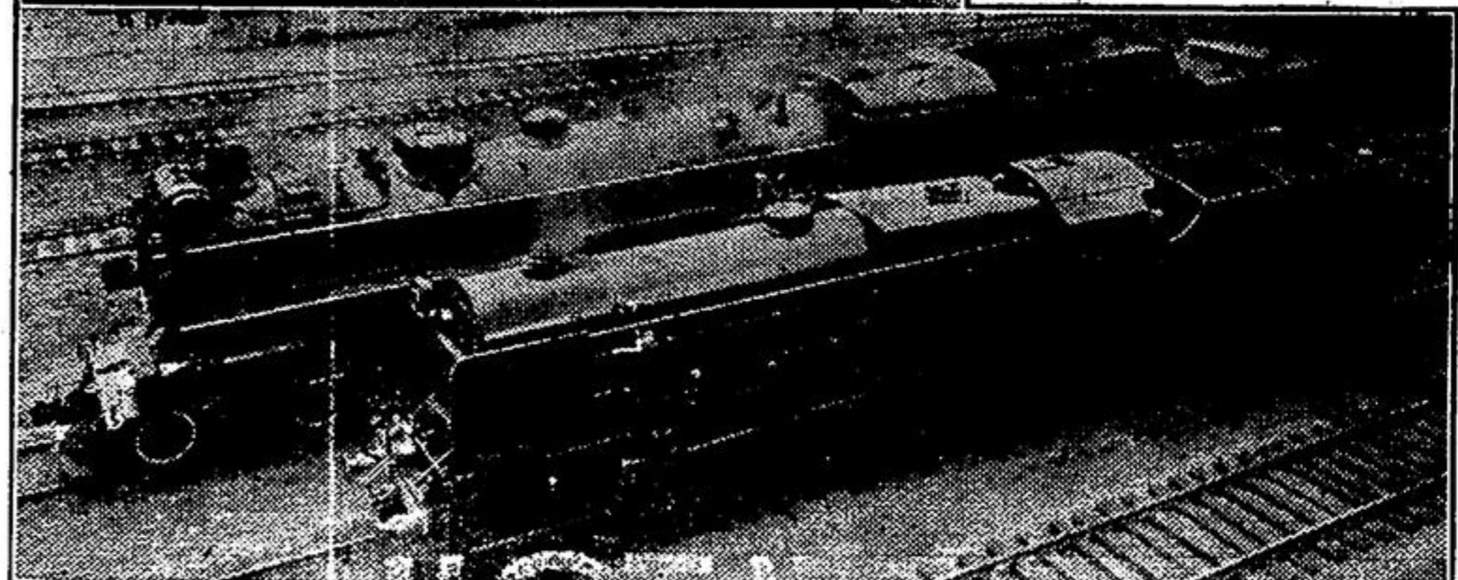
The Royal Scot, here from Great Britain to haul the flyer of the London, Midland & Scottish Railway on its Canadian and United States tour, and Number 2810 of the Canadian Pacific's fleet of flyers, comparing notes and doing a little boasting at the Canadian Pacific's Angus Shops, Montreal. The Royal Scot has been equipped with a bell and searchlight to meet North American railway regulations.
