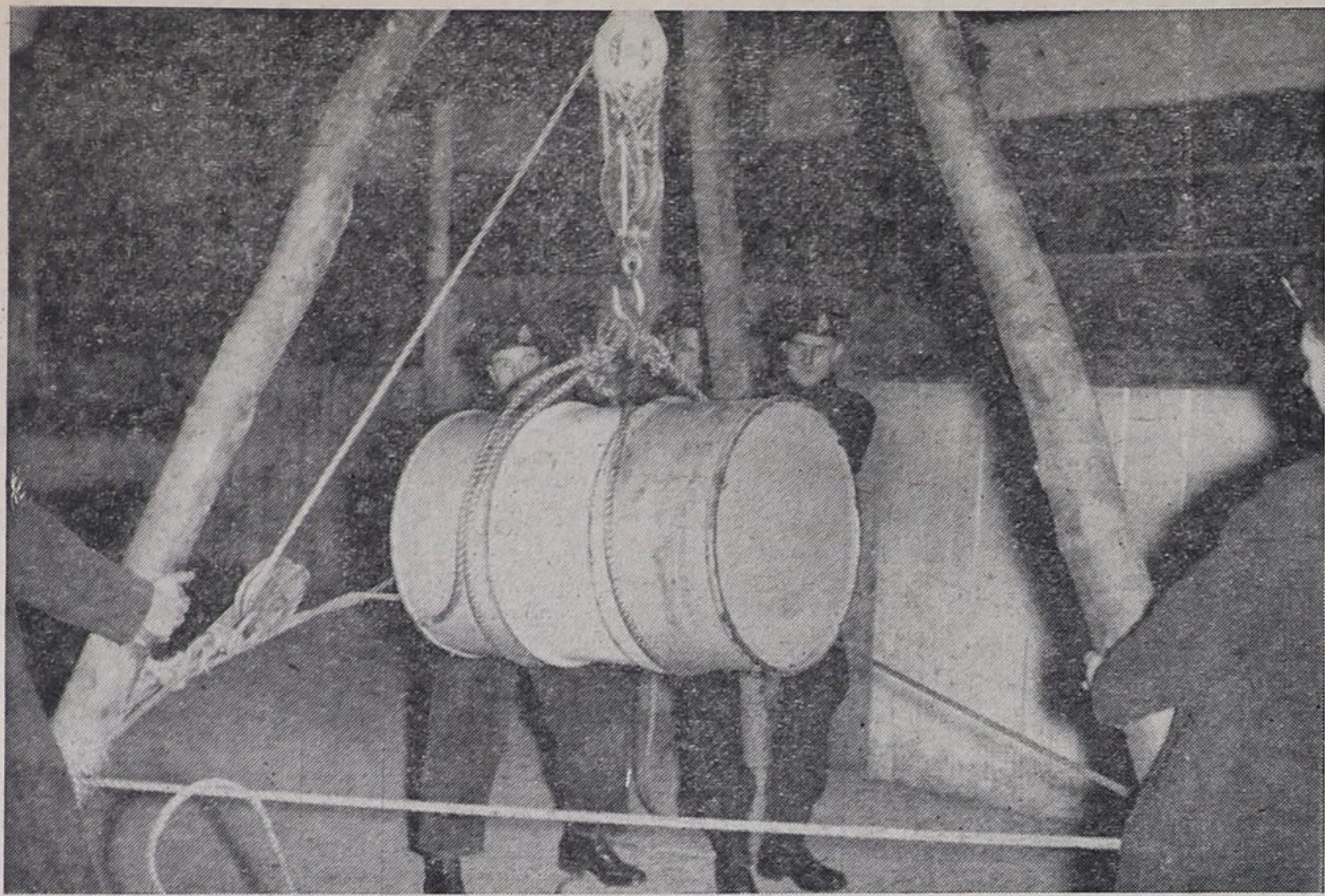
Using a full barrel of oil, the Rescue Squadron of the Algonquin Regiment demonstrates how to lift an injured man from a shaft using a tripod, block and tackle and sling.
