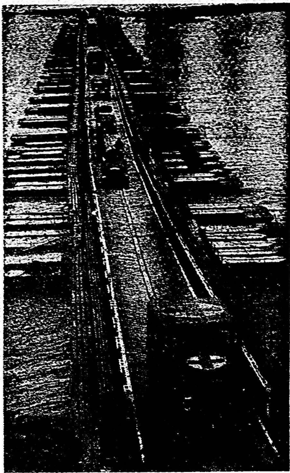
Built by Canadian Army engineers, this Bailey Bridge across the Rhine is shown shortly after it was opened to traffic. The small sign in the left foreground tells the distance that must be maintained between each vehicle so as not to overload any one portion of the bridge.
