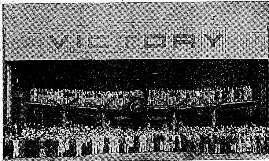
Here is the 300th Lancaster bomber leaving the assembly line of the Victory Aircraft plant at Malton, Ontario. This Crown company is producing one of these planes a day. Loaded, the plane weighs 30 tons. It has a speed of some 300 miles an hour, a range of 3,000 miles, and an eight ton bomb load. Its armament includes 10 machine guns mounted in revolving turrets. Its record as a bomber has not been equalled by any other aircraft.
