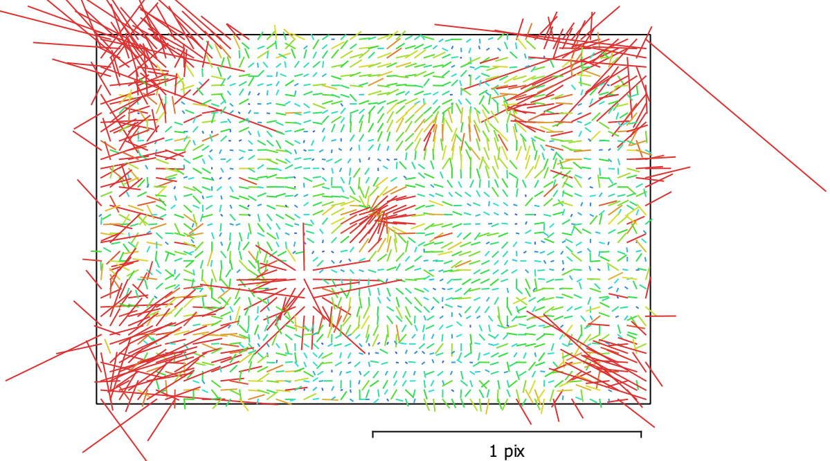
Fig. 2. Image residuals for Canon EOS 5D Mark IV, EF8-15mm f/4L FISHEYE USM (15mm).
