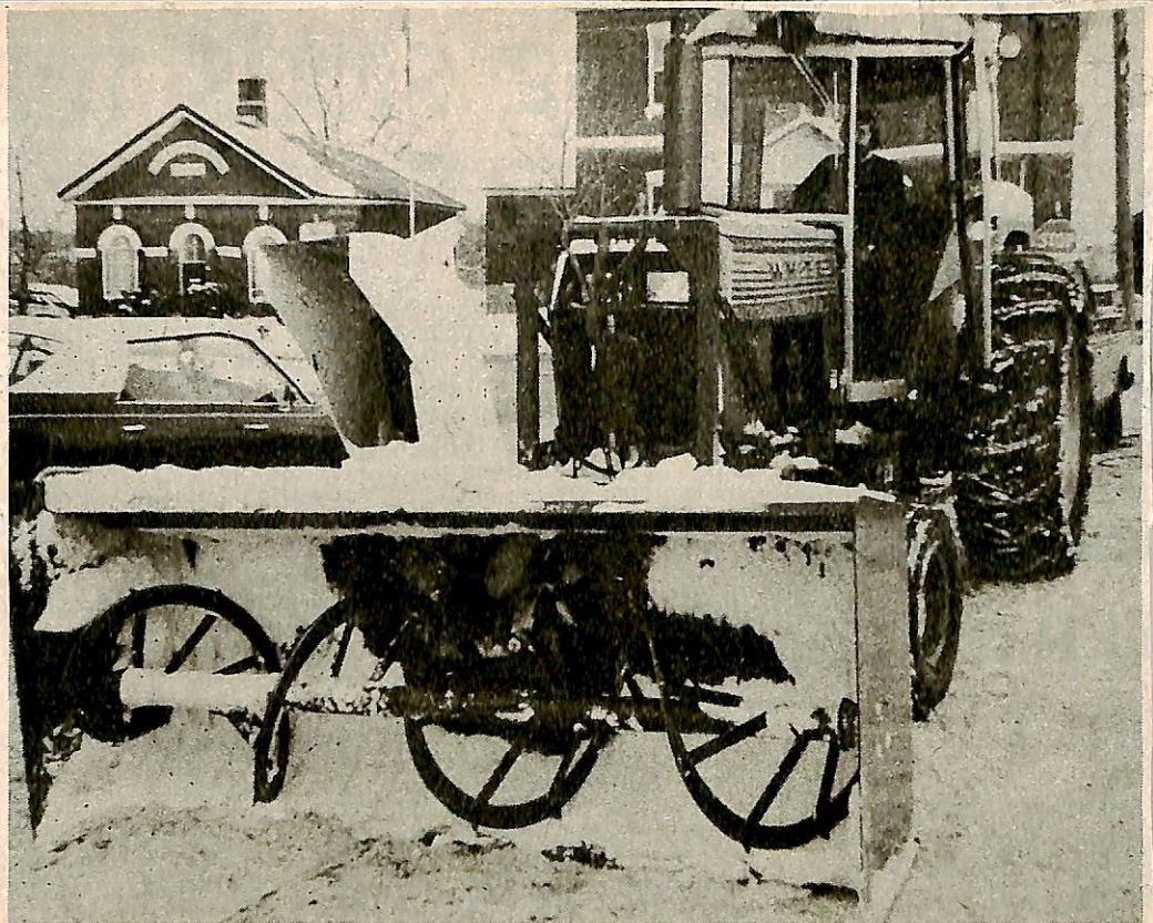
A BLOW FOR SNOW .... This eight foot model front mounted snow blower is unique to Prince Edward County. Owner Harold Bartman of RR 2, Milford, says it cost him $4,500 and was supplied by Eastern Farm Machinery. The blower is powered by a 85 hp White tractor. Mr. Bartman's son David Grimmon operates the equipment and is kept busy clearing driveways and parking lots of snow.
