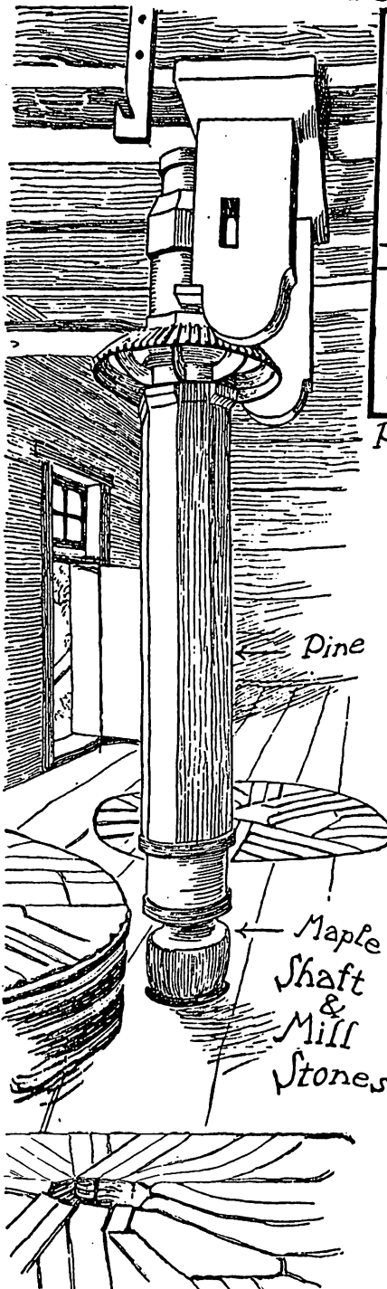
Sectional Diagram of Water Power Transmission
