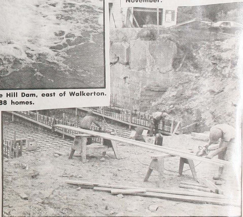
THE HYDRO PROJECT AT MAPLE HILL is going along on schedule and work should be complete by November. Doing the construction work is Owen King Construction Limited, of Walkerton.
