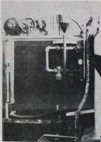
The above photograph shows the facilities of Kincardine P.U.C. in 1920. A steam powered pump in the background and new electric powered pump in the foreground. PHOTO BY FRED HOLMES 1920. Pictured on the right side is the first ever chlorinator used by the Kincardine P.U.C. and was built by Fred Holmes.
