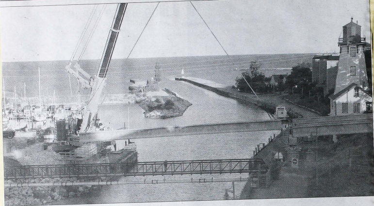
A huge crane arrived in Kincardine last Tuesday evening to lift the 60 tonne support beams for the new Huron Terrace bridge into place. Above, the first one is being dropped into place about 7:30 a.m. Wednesday. The work attracted a large crowd of sidewalk superintendents. (Eric Howald photo)
