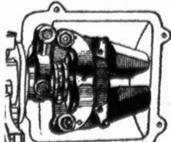
Governor
