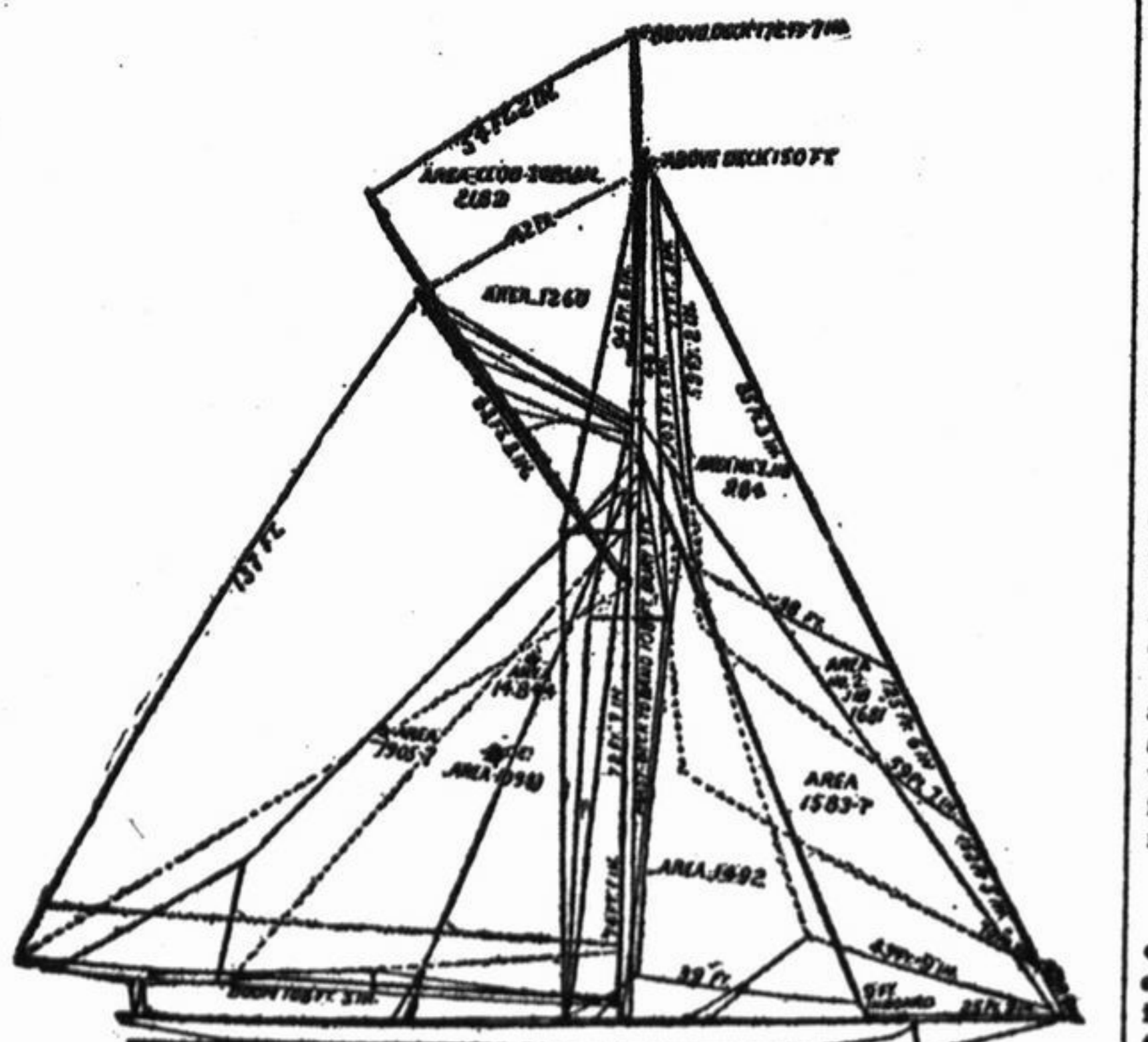
SAIL PLAN OF T. W. LAWSON'S NEW YACHT INDEPENDENCE.
