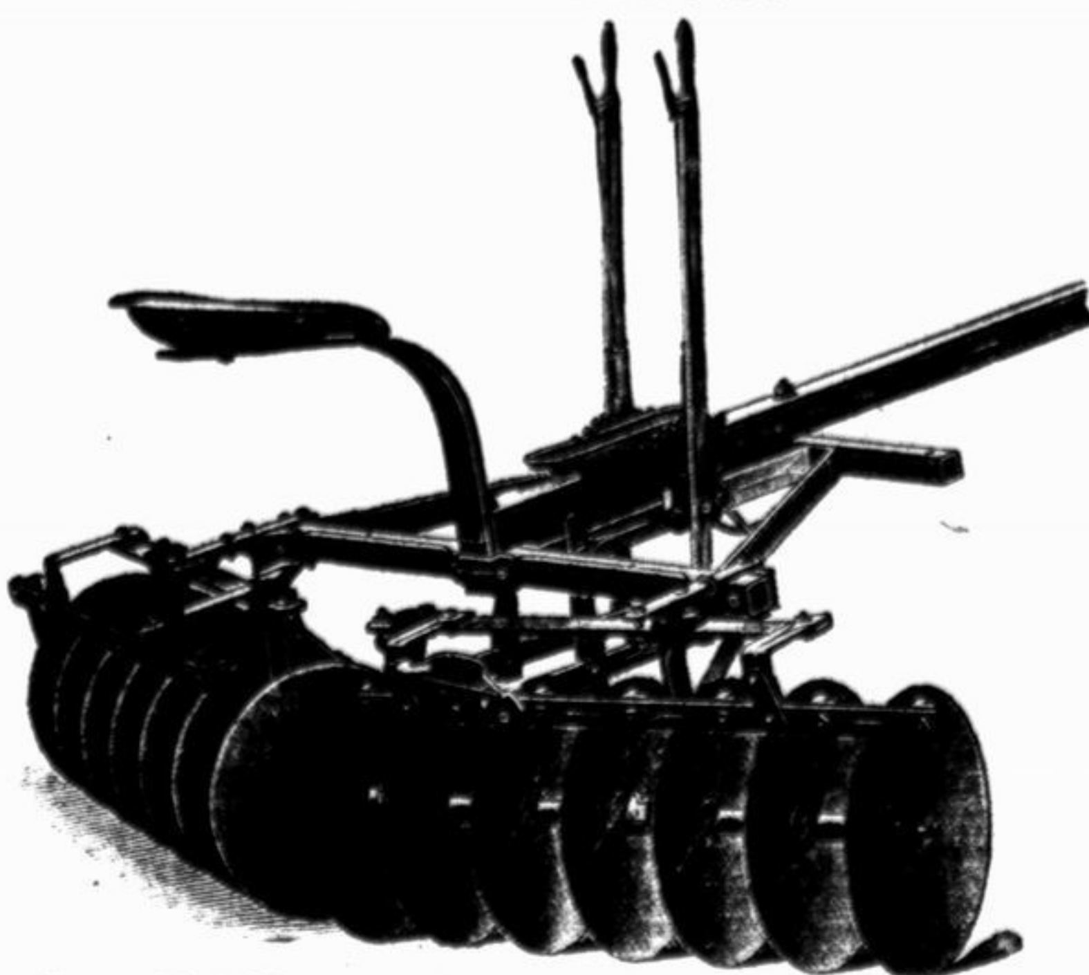
Steel frame Disk Harrow, with 12, 14 and 16 inch disks. 6 1/2 and 7 1/2 ft. cut. Two levers, one for each gang disks. Other good features.
