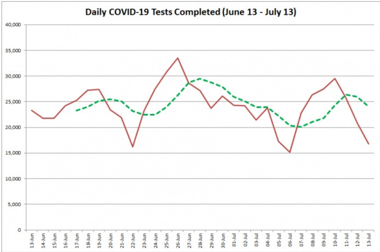
COVID-19 tests completed in Ontario from June 13 – July 13, 2020. The red line is the number of tests completed daily, and the dotted green line is a five-day moving average of tests completed. (Graphic: kawarthaNOW.com)
