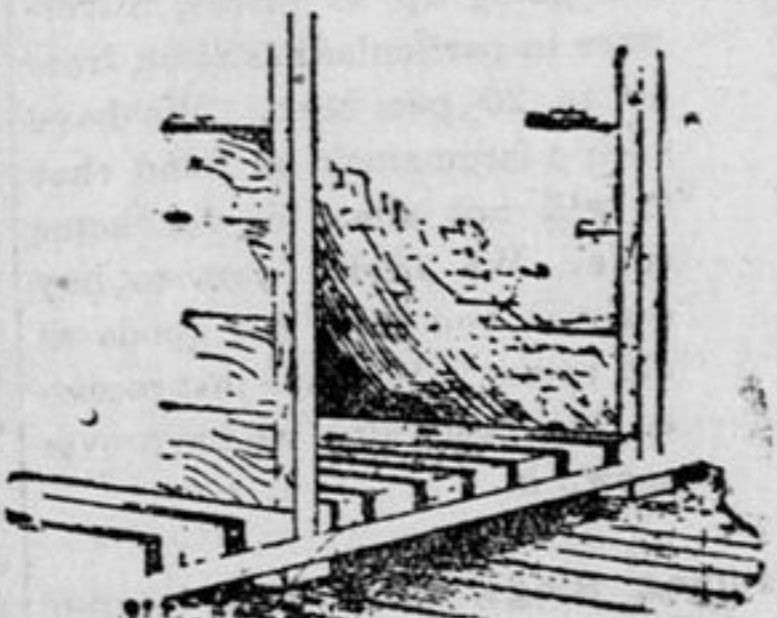
FLOOR FOR HORSE STALLS. which the stall floor is made may be five inches wide laid one-half inch apart. They are shown farther apart than this in the cut in order to make the matter plain. There should be four cross bearings under the stall floor if two-inch stuff is to be used.
