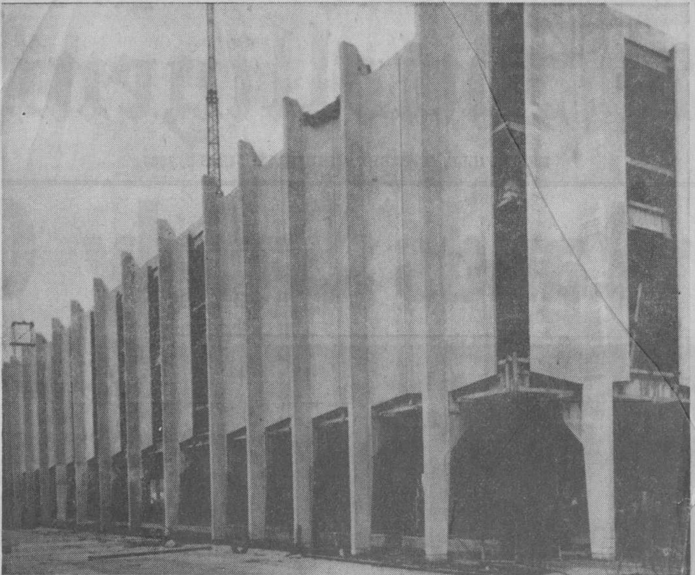
SCHOOL CHOSEN AS EXHIBIT BY LOCAL FIRM — Photos of the new High School of Commerce in Ottawa, a current project of Wilson Concrete of Belleville, have been chosen by the local firm to be sent as an exhibit to the 1966 International Prestressing Federation Congress in Paris.
