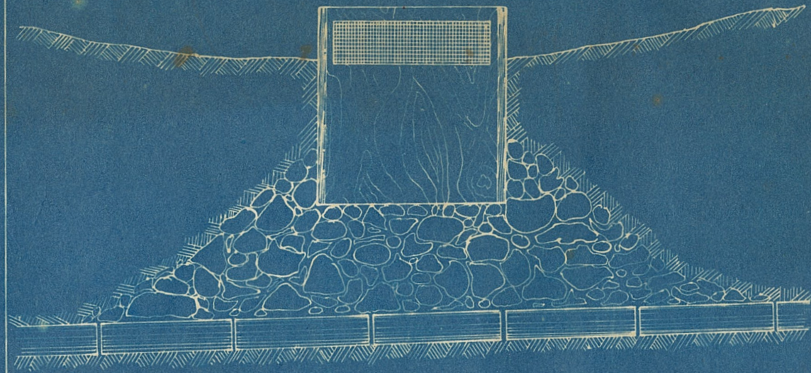
SECTION OF STONE SINK AND FILLER WITH SCREENED BOX INTAKE. FIGURE 3
